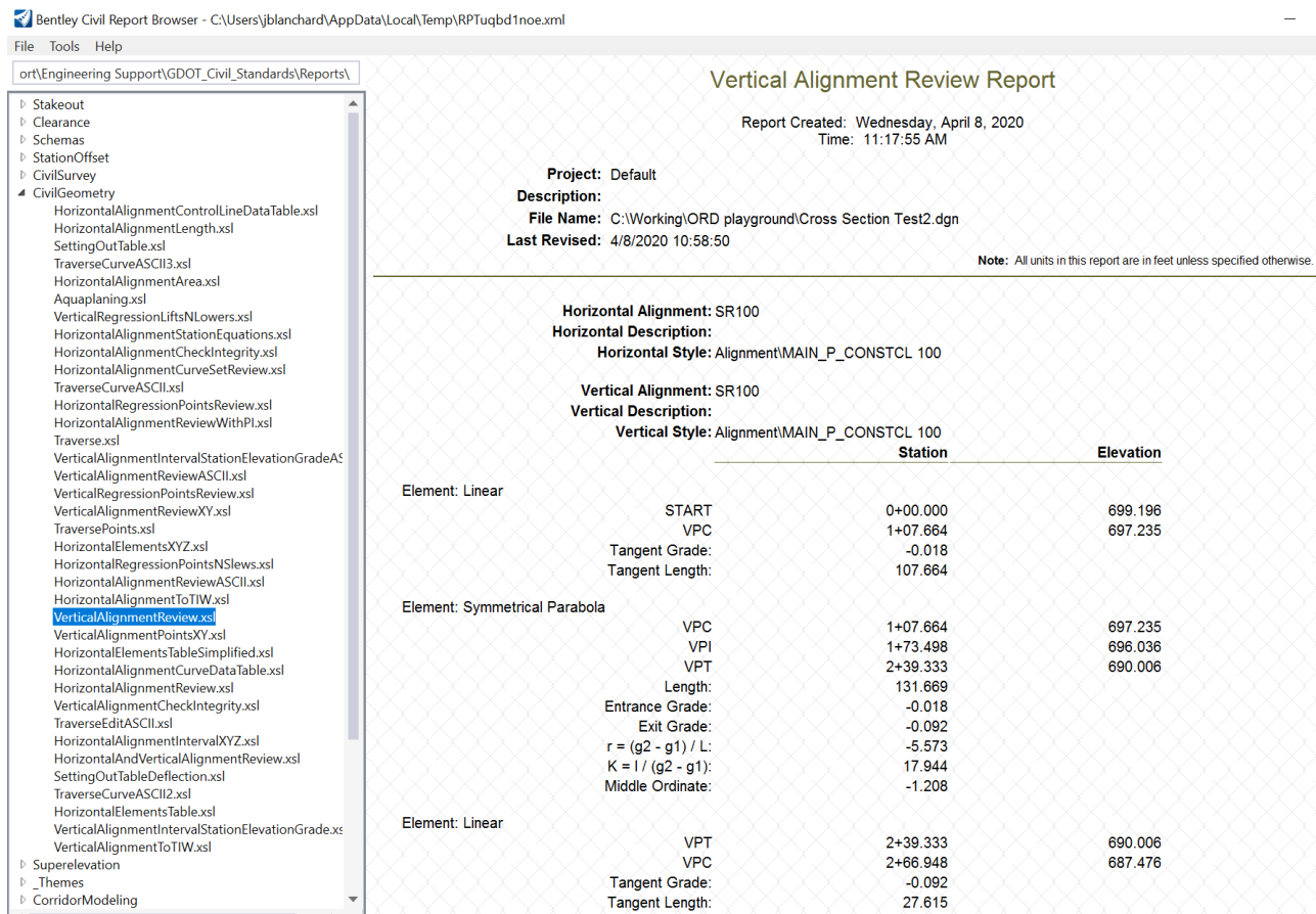
Figure 4-1 Review Vertical Alignment
